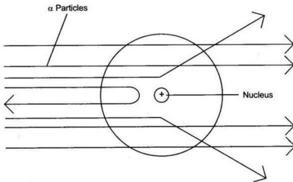
Rutherford's Model
