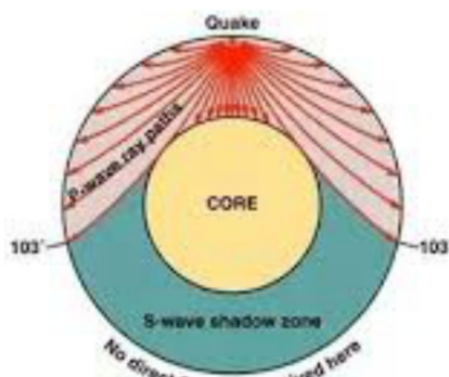
S-wave shadow zone = 154^\circ
