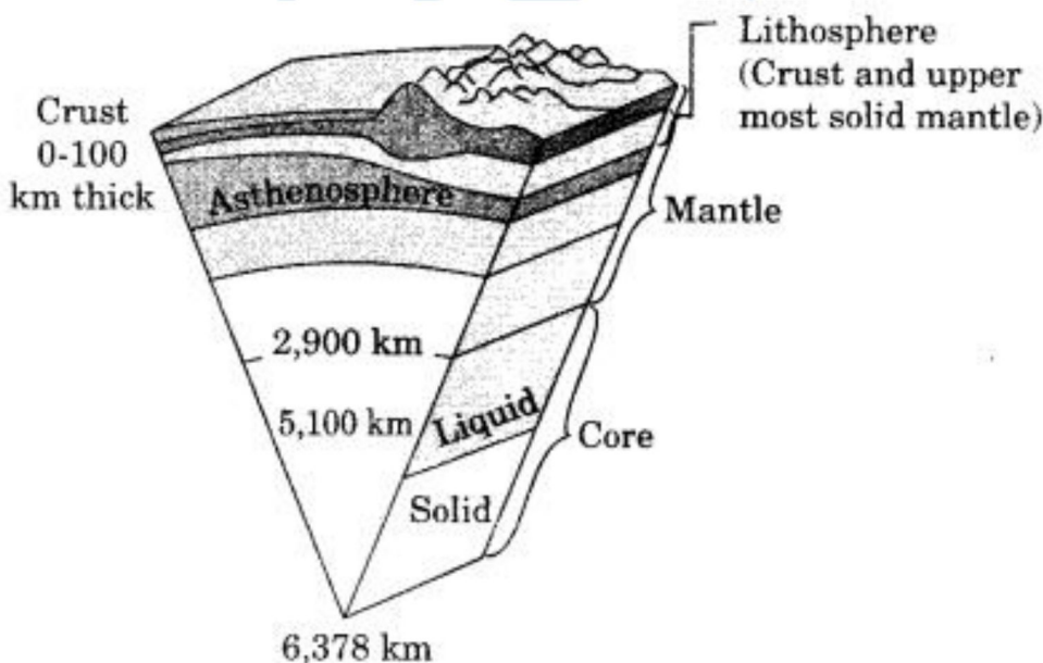
Fig: The interior of the earth
