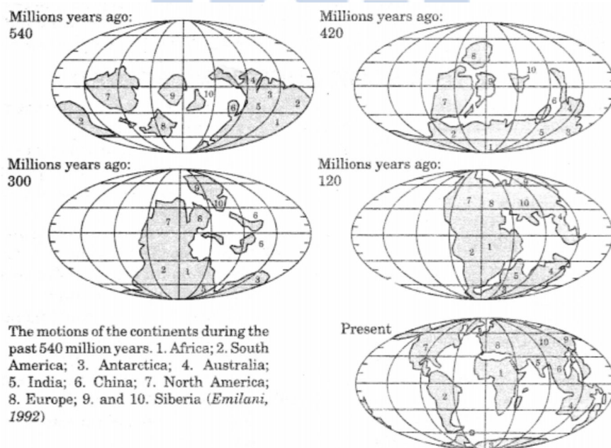
Fig: Position of continents through geological past
